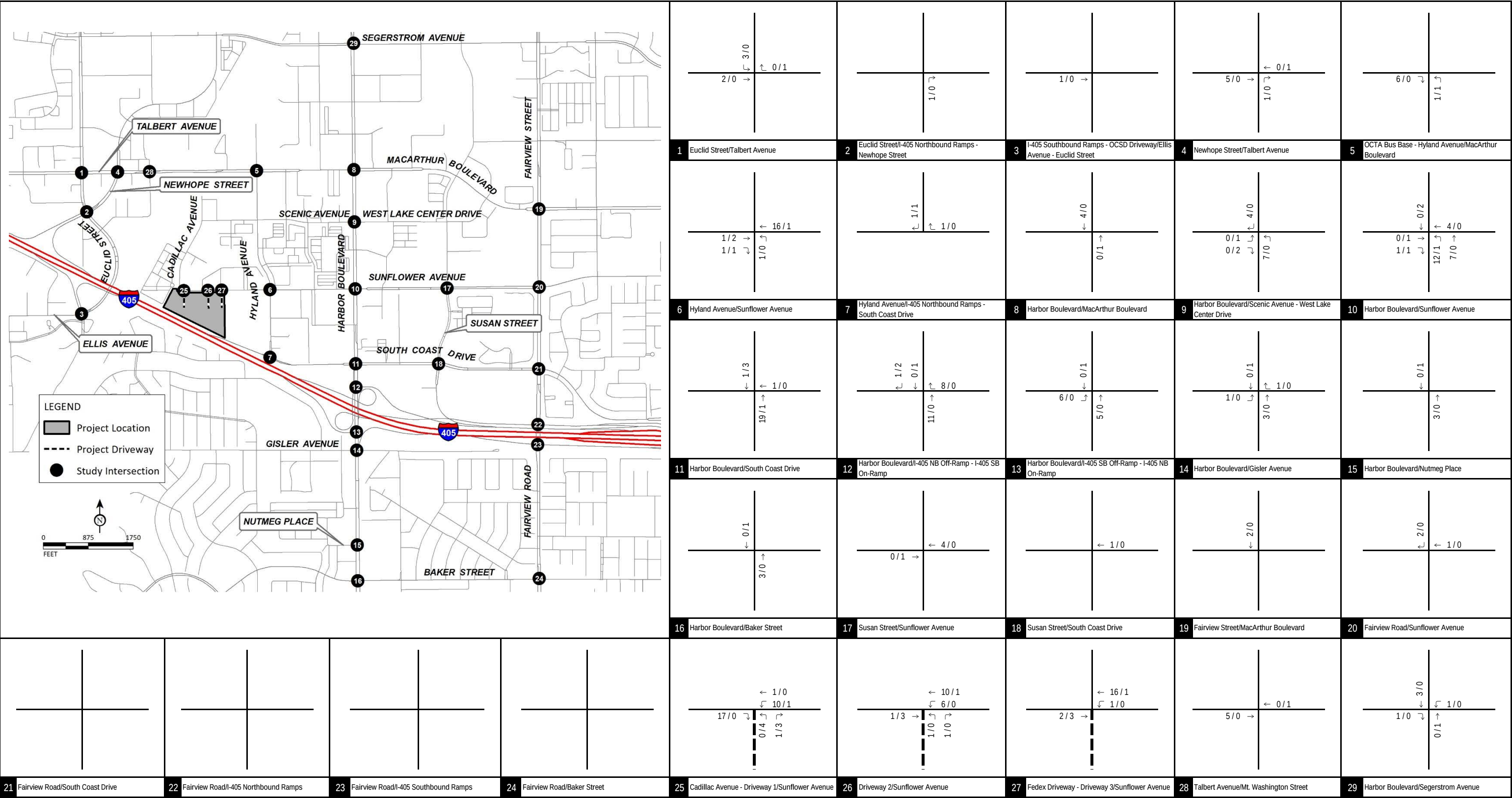
LSA XX / YY AM / PM Peak Hour Traffic Volumes -- Project Driveway One Metro West Traffic Impact Analysis Trip Assignment - Existing Use FIGURE 5-4
